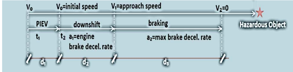
Figure 1 MSSD Scheme
