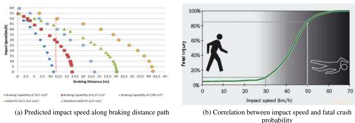
Figure 3 Effect of decreased speed due to downshifting on the braking distance and impact speed
