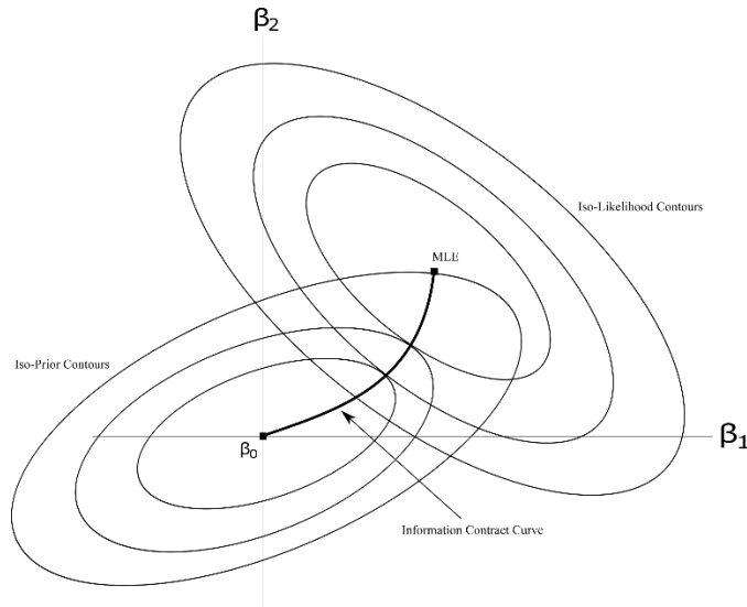
Figure 1 Likelihood/Prior Contours & Information Contract Curve
